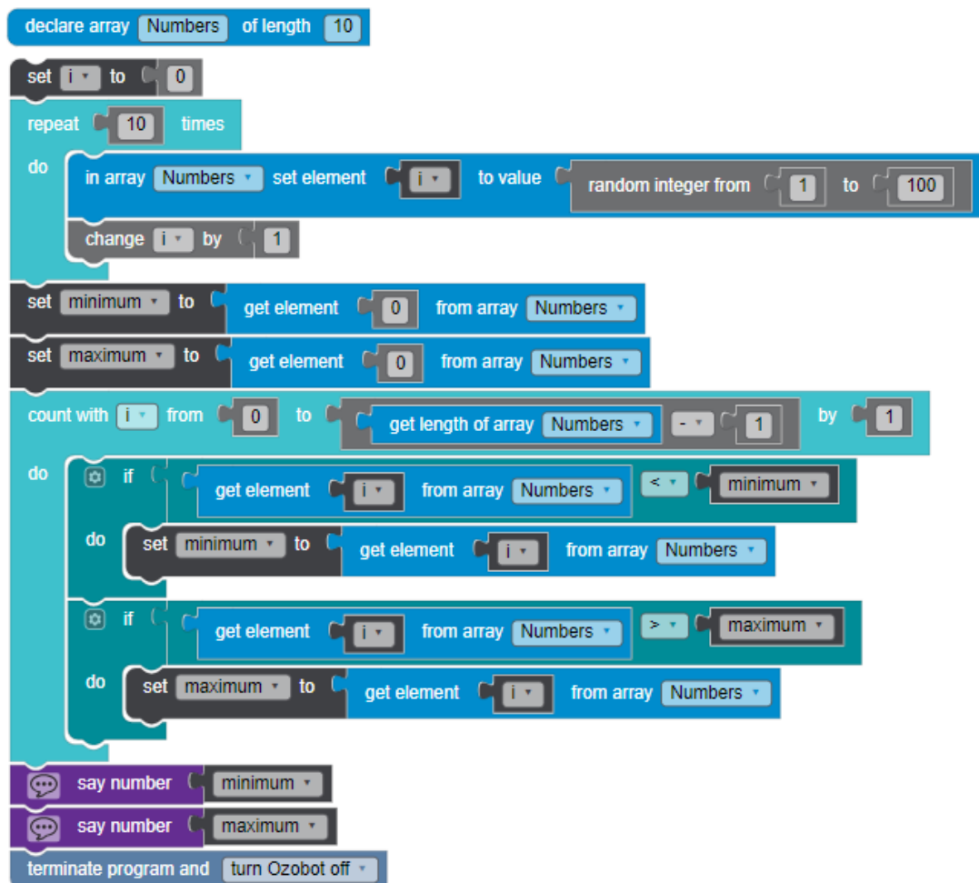
Figure 5 Example program for the extension
