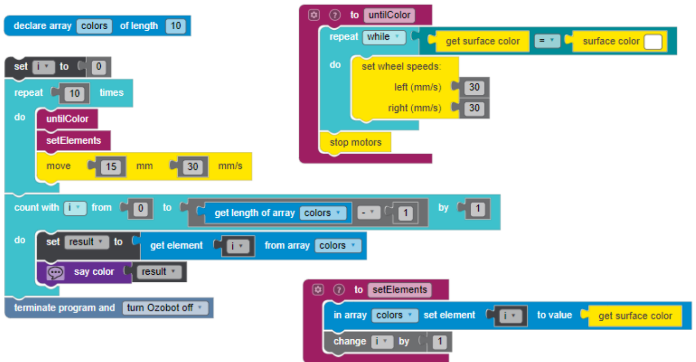
Figure 3 Line counting program with arrays
