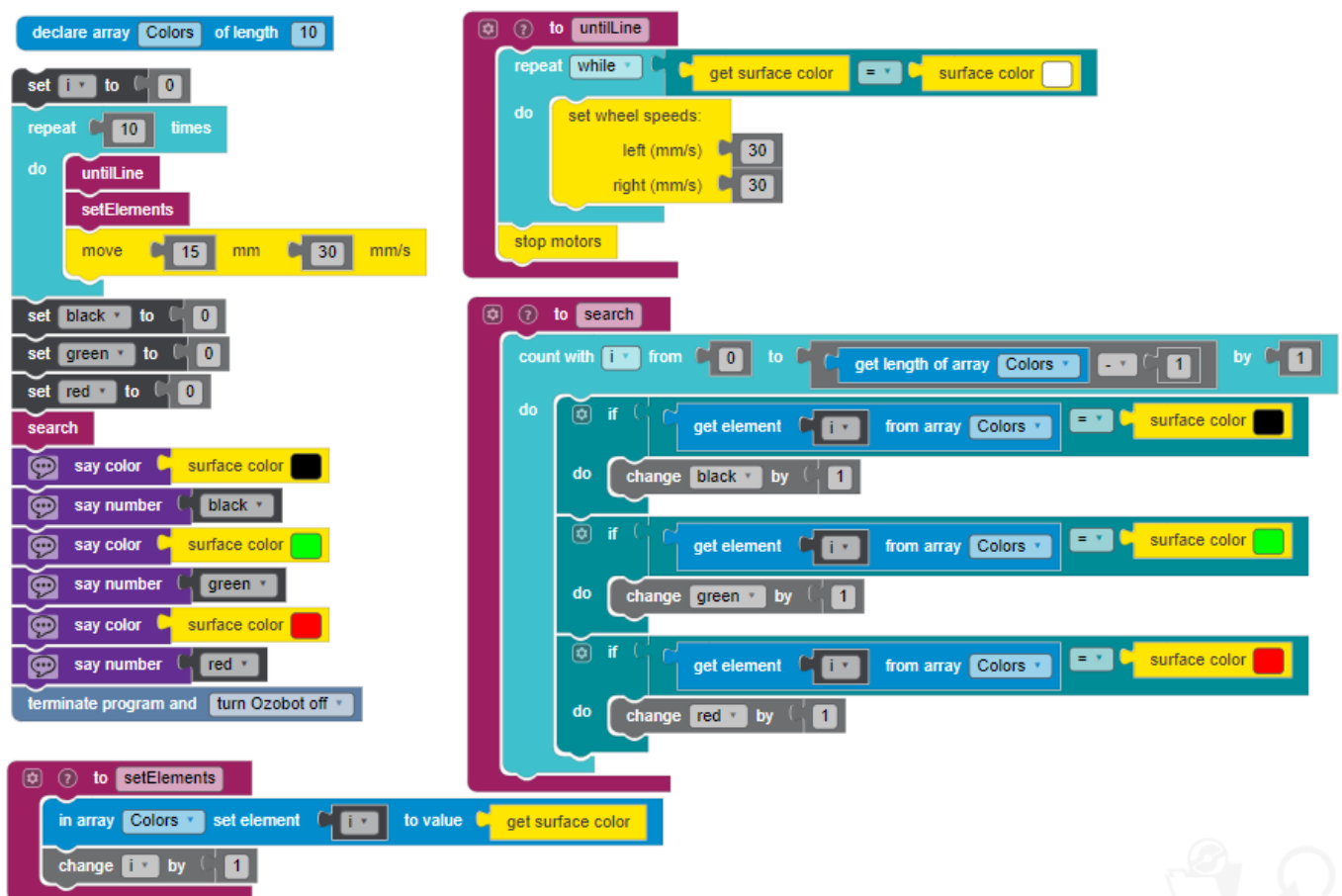
Figure 4 Search and count colors in the array
