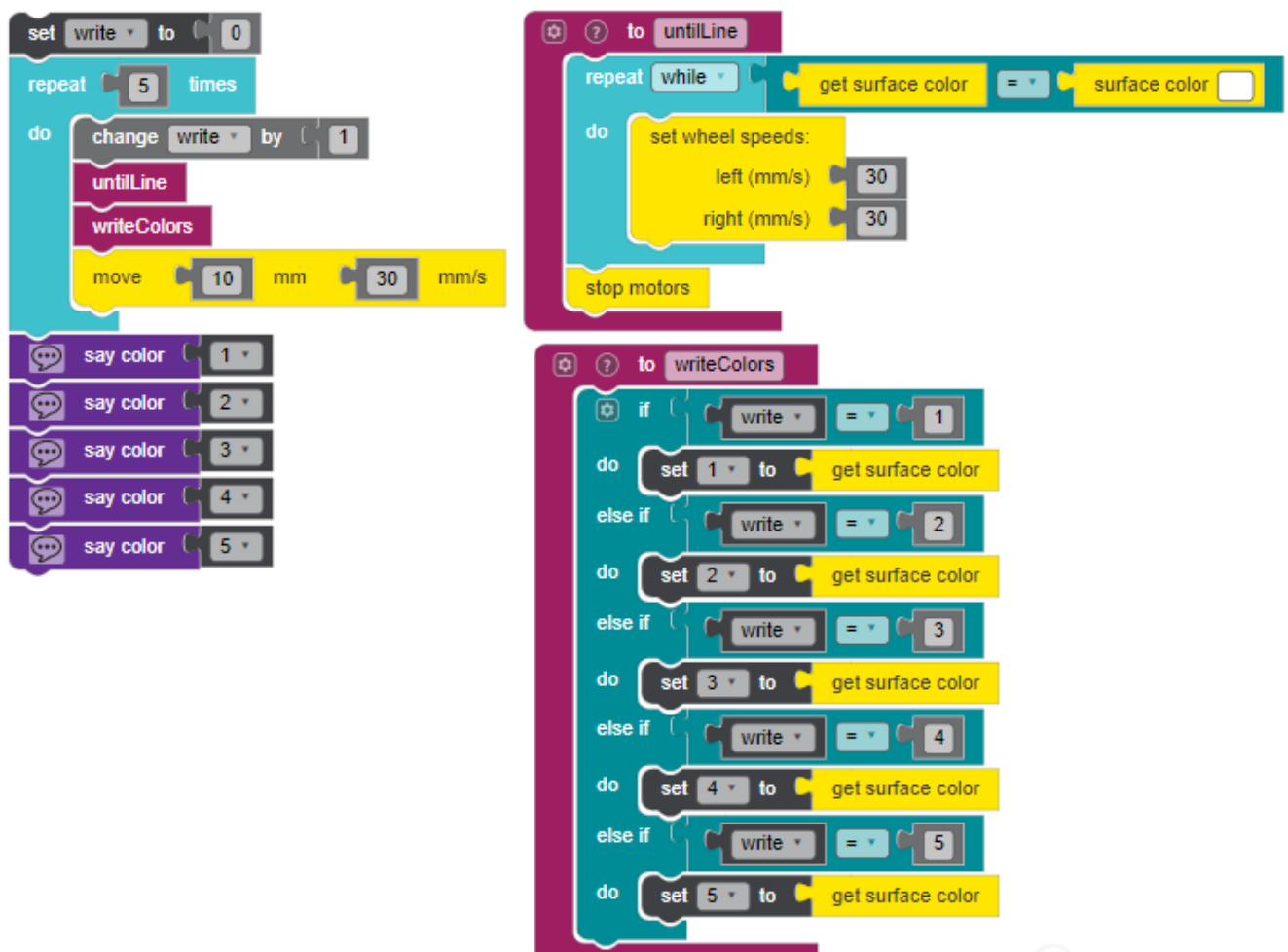
Figure 2 Line counting program with variables
